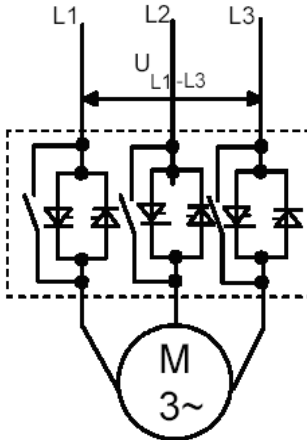
5-2 Bypass- Kontakte
